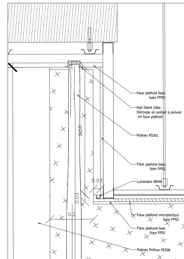
DETAIL 3 - 1/5 ème DETAIL 1007-02
