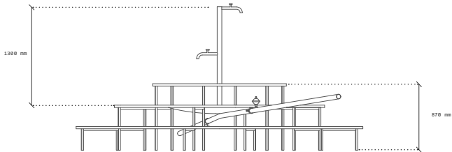
Elevation 1/20
