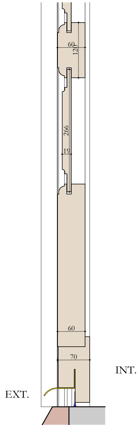
Section verticale BB
