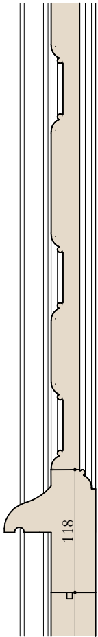
Section verticale CC
