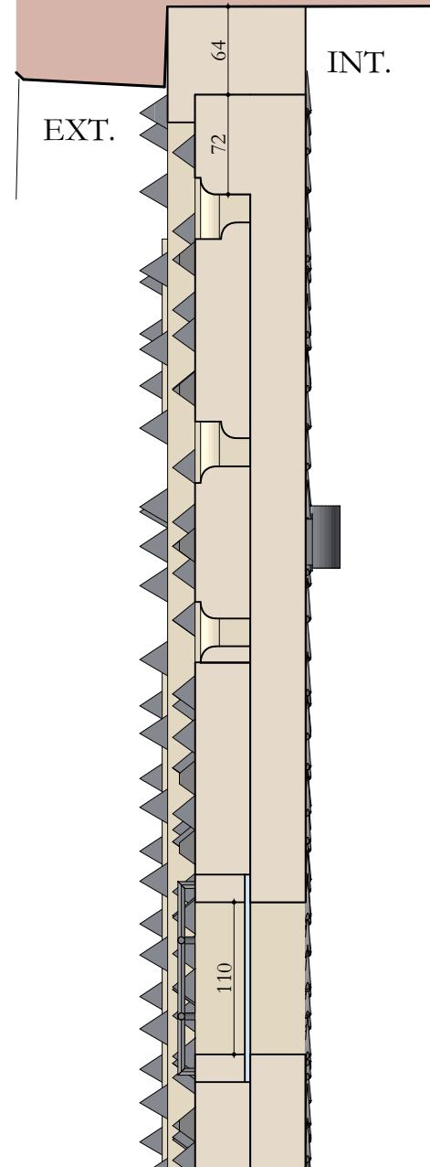
Section verticale CC
