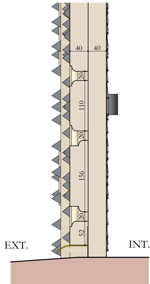
Section verticale BB
