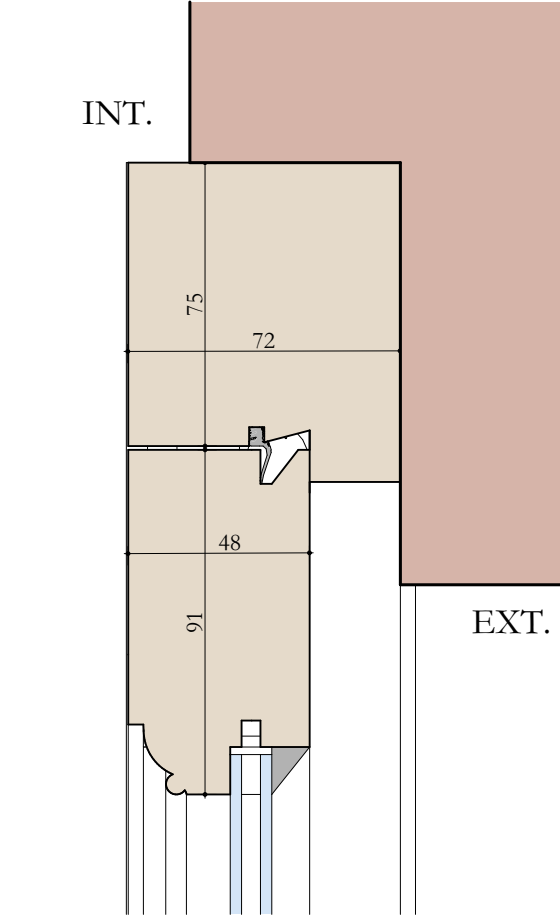
Section verticale CC
