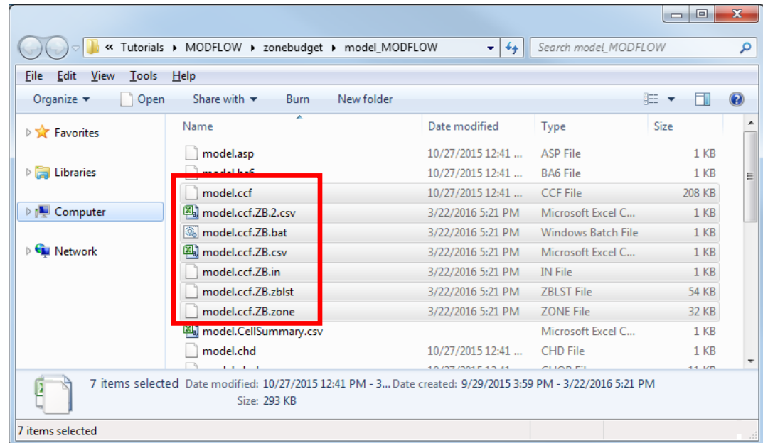
Figure 4 ZONEBUDGET input and output files
