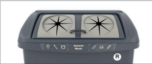
SELECTIVE OPENINGS – Circular openings, Ø200 and Ø400, and paper opening 975 x 200 mm
